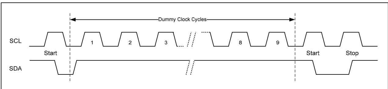
Figure7 Soft Reset
