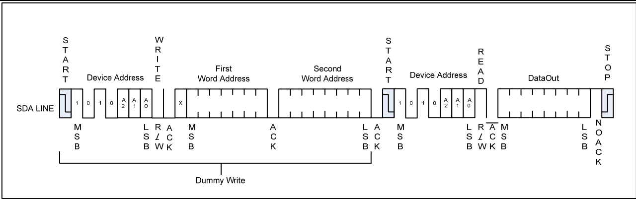
Figure12 Random Read
