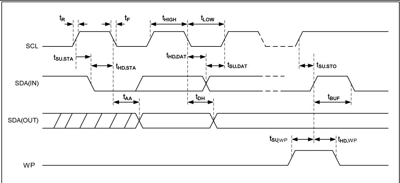
Figure2 Bus Timing
