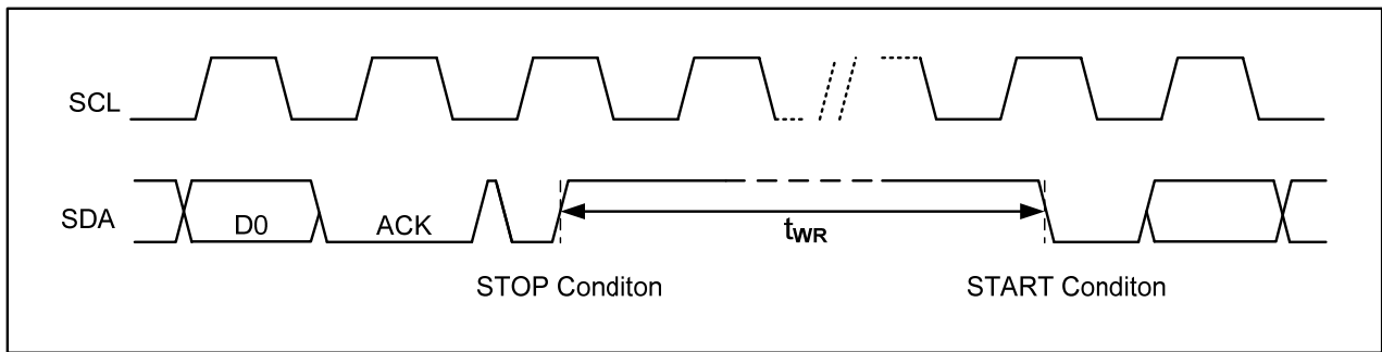
Figure2 Bus Timing
