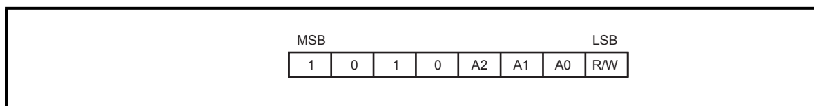
Figure8 Device Address
