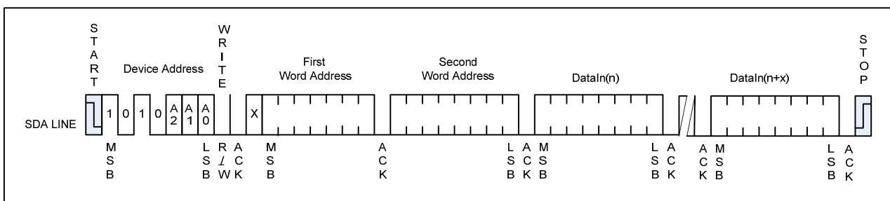
Figure10 Page Write
